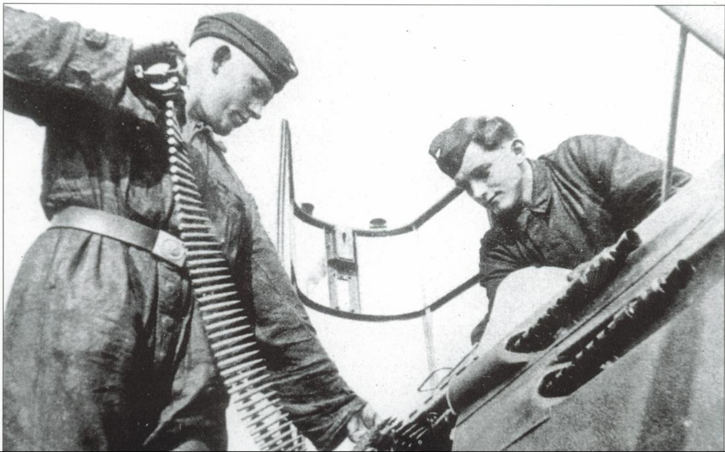
Below: Luftwaffe armourers carefully load a belt of 7.9mm bullets into a machine gun mounted alongside the nose of a German fighter. Care is essential if the pilot is not to be plagued by stoppages in mid-combat – a potentially fatal occurrence.
