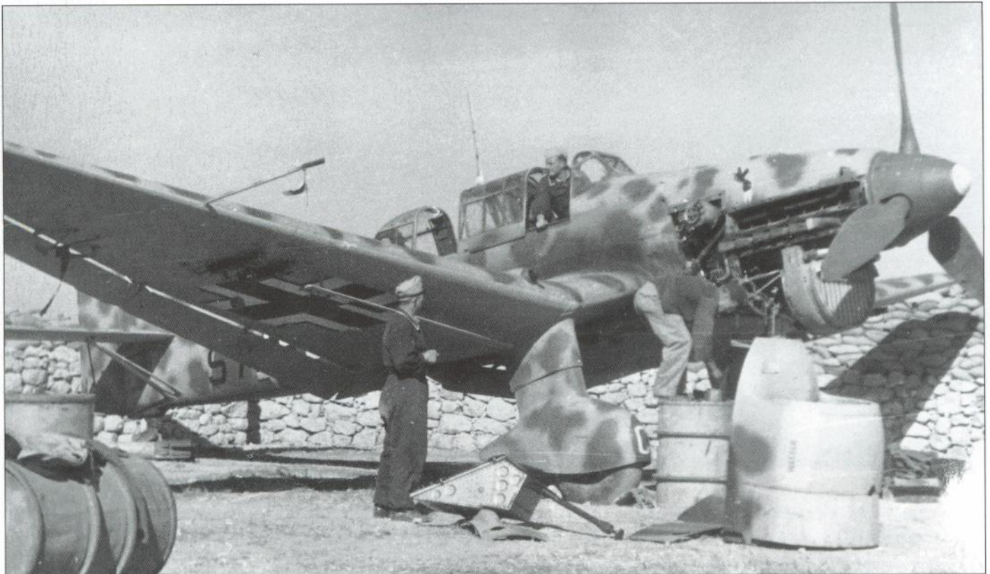
Below: Mechanics work on the Junkers Jumo 211Da 12-cylinder liquid-cooled engine of a Ju 87B. This particular aircraft has been 'tropicalised' by the addition of sand filters.
