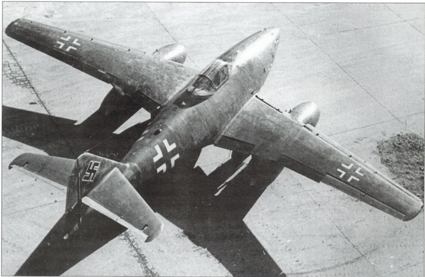
Above: The lack of unit markings suggests that this is a pre-delivery example of the Messerschmitt Me 262 jet fighter. The slightly swept-back wings and nacelles for the two Junkers Jumo 004B axial-flow turbojets are shown to advantage.
