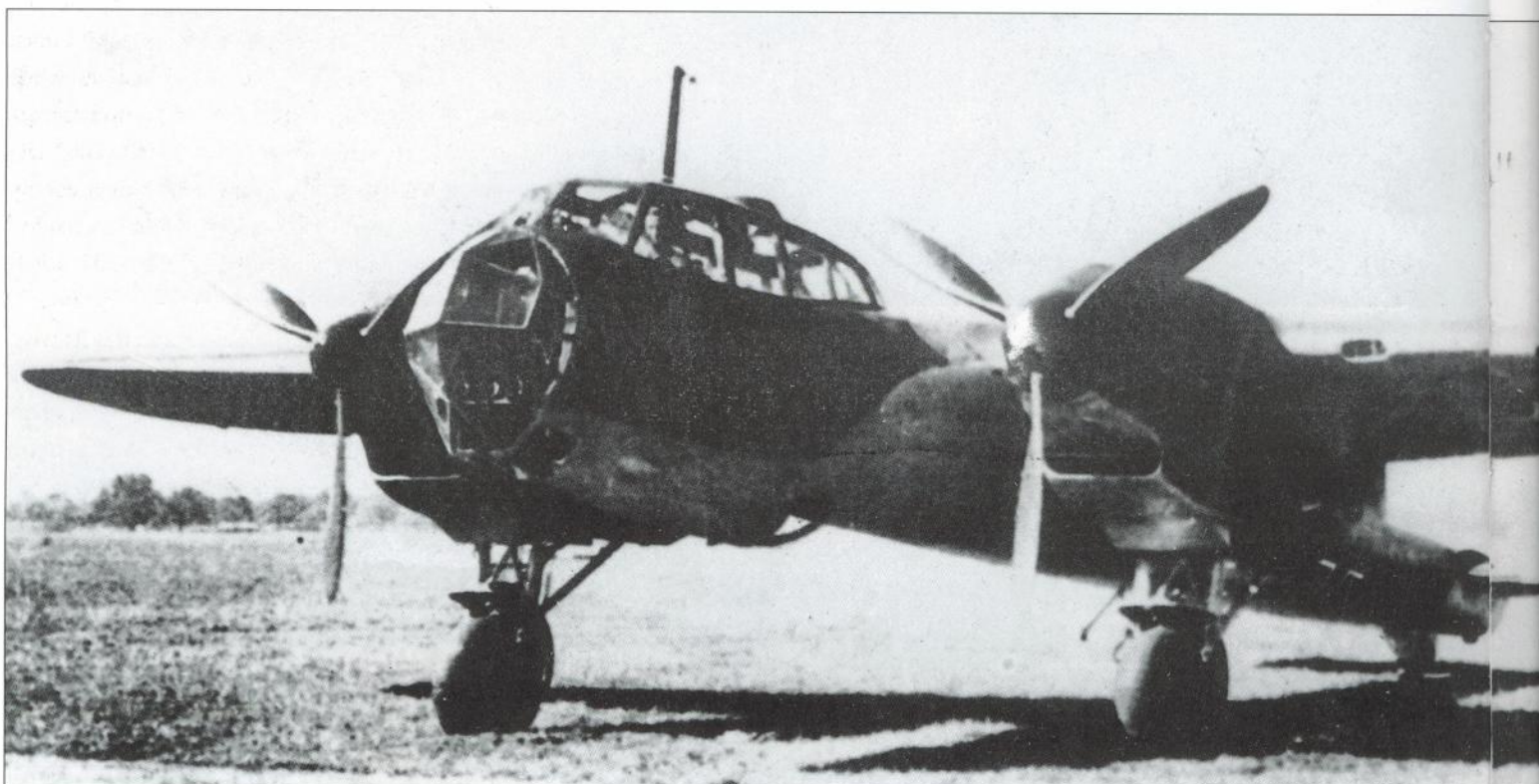
Below: A Dornier Do 17S high-speed reconnaissance aircraft. The Do 17S was powered by two Daimler-Benz DB 600G liquid-cooled engines, but did not enter squadron service. The engines were diverted to the fighter programme, leaving subsequent Do 17s to make do with BMW-Bramo 323 radials.
