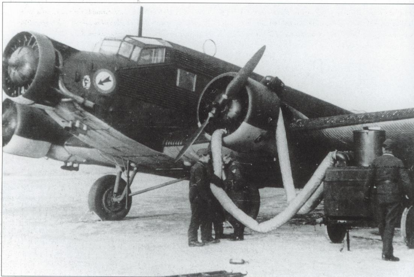
Below: A Junkers Ju 52 transport is prepared for take-off on an airfield on the Eastern Front, winter 1944-45. The pipes into the port nacelle carry hot air to warm the engine.
