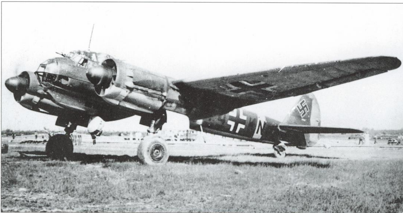
Above: A Junkers Ju 88A runs up its engines on an airfield in the Soviet Union, 1941. With a maximum speed of 467kmph (292mph) and operational range of more than 1600km (1000 miles), the Ju 88 was a useful medium bomber, but its bomb-carrying capacity was limited to 1818kg (4000lb).
