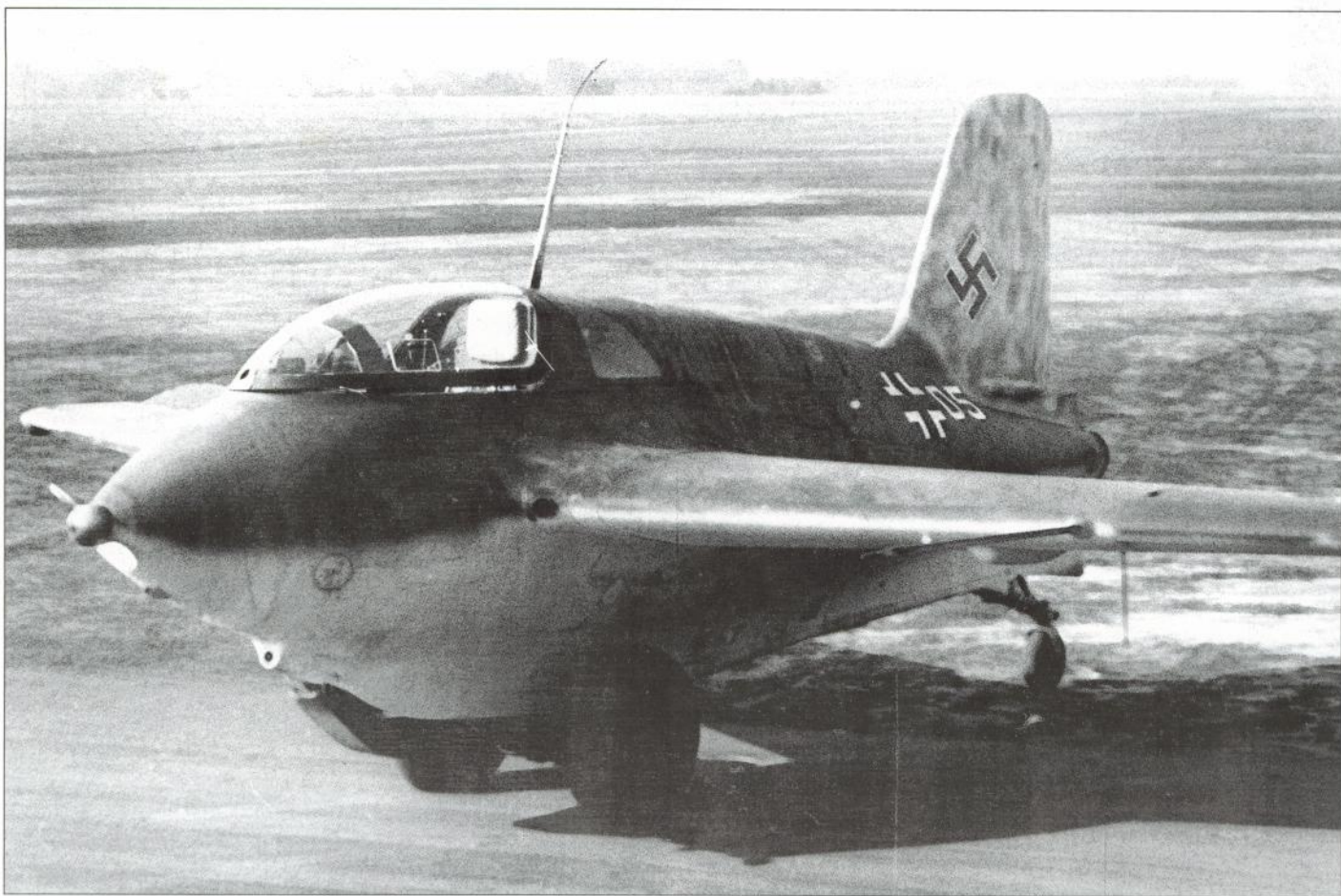
Below: A standard production Messerschmitt Me 163B-1a, 1945. It was an impressive machine, but its unstable fuel and short flying duration seriously undermined its effectiveness.
