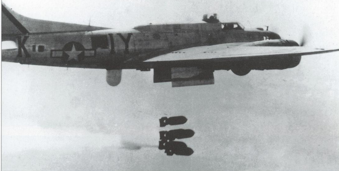
Above: Part of the bomb-load of a Boeing B-17 Flying Fortress bomber begins its descent onto a target in Germany, 1944. The 'dustbin' beneath the fuselage is an H2X radar radome, installed in place of the normal ball turret, indicating that this particular aircraft is a pathfinder.
