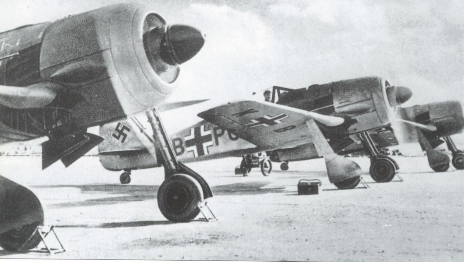
Above: The three Focke-Wulf Fw 190A-0s of the manufacturer's flight test line run their engines, summer 1941. In the foreground is a 'small-wing' variant, with two 'large-wing' versions behind. The Fw 190 performed well as a fighter.
