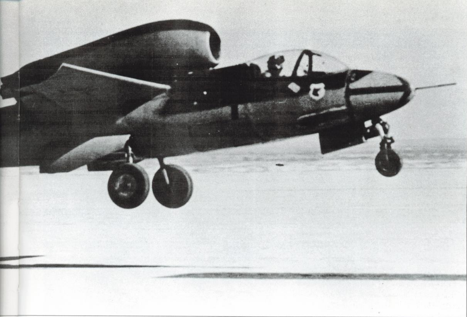
Above: A Heinkel He 162 single-seat jet fighter takes to the air. This aircraft, captured in May 1945, was shipped to the United States for flight evaluation, where this photograph was taken. The nose markings suggest that it served in Jagdgeschwader 1.
