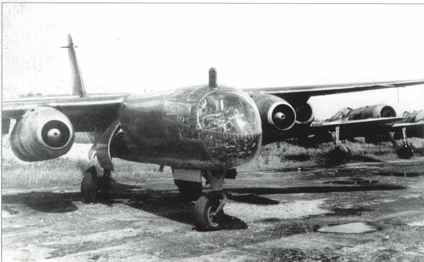
Below: An Arado Ar 234B abandoned on a German airfield. The fixed undercarriage is an improvement on the 'A' series. The engines are Junkers Jumo 004B Orkan axial-flow turbojets.
